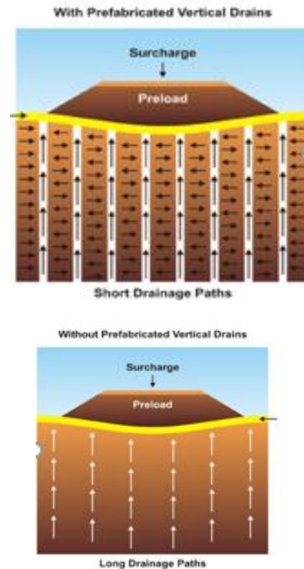
Fig.2 Cross-Section Without and With Vertical Drains
