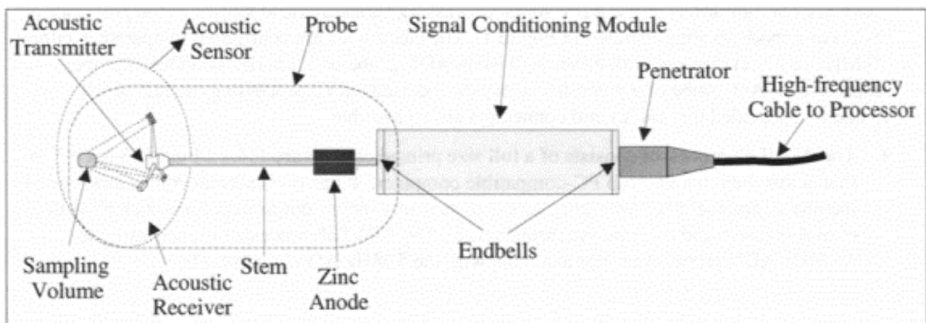
Figure 1: Schematic of Sontek ADV probe (Courtesy: Sontek)
