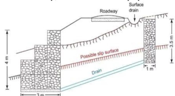
Fig. 7: Gabion retaining wall for road embankment
