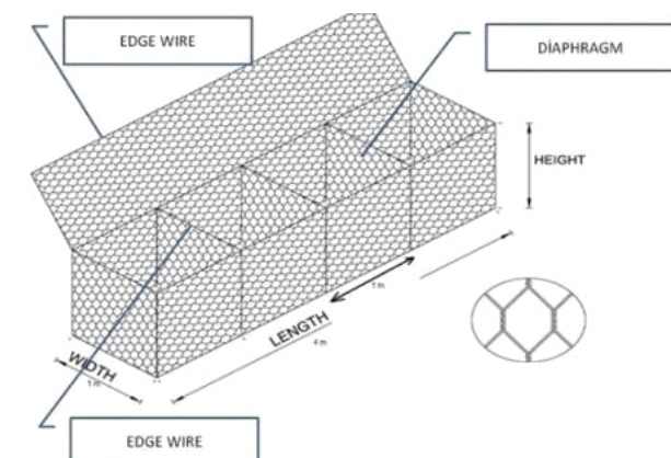
Fig. 1: Wire mesh boxes for gabions
