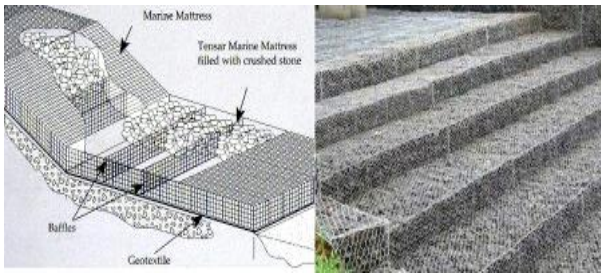
Fig. 3: Gabion mattress
