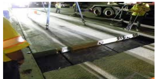
Fig.4 Post-tensioned system
