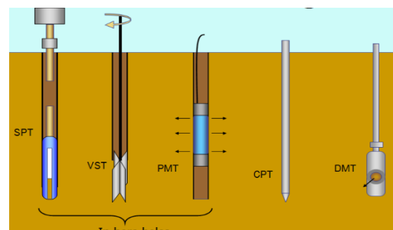
Figure 2: Various types of soil investigations
